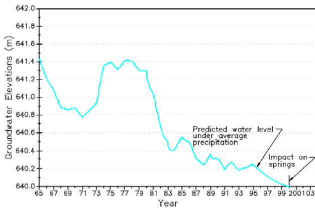
Figure 10c: Predicted Water Level Trends
