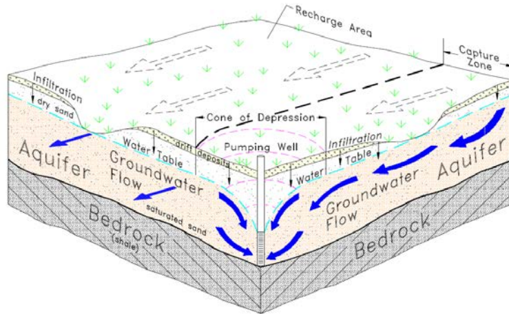
Figure 8: Well Capture Zone
