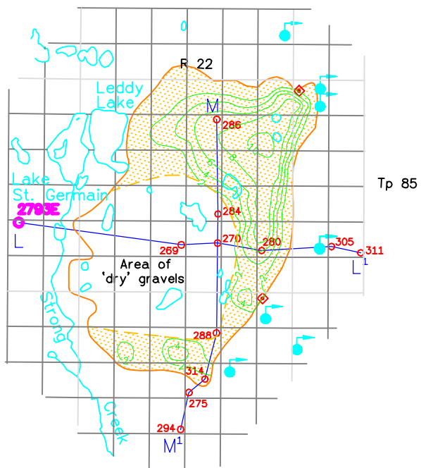
INTERPRETED SATURATED THICKNESS
