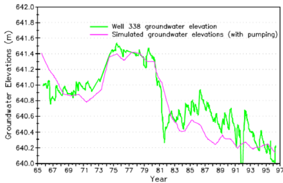
Figure 9b: Simulated Water Level Data with Pumping
