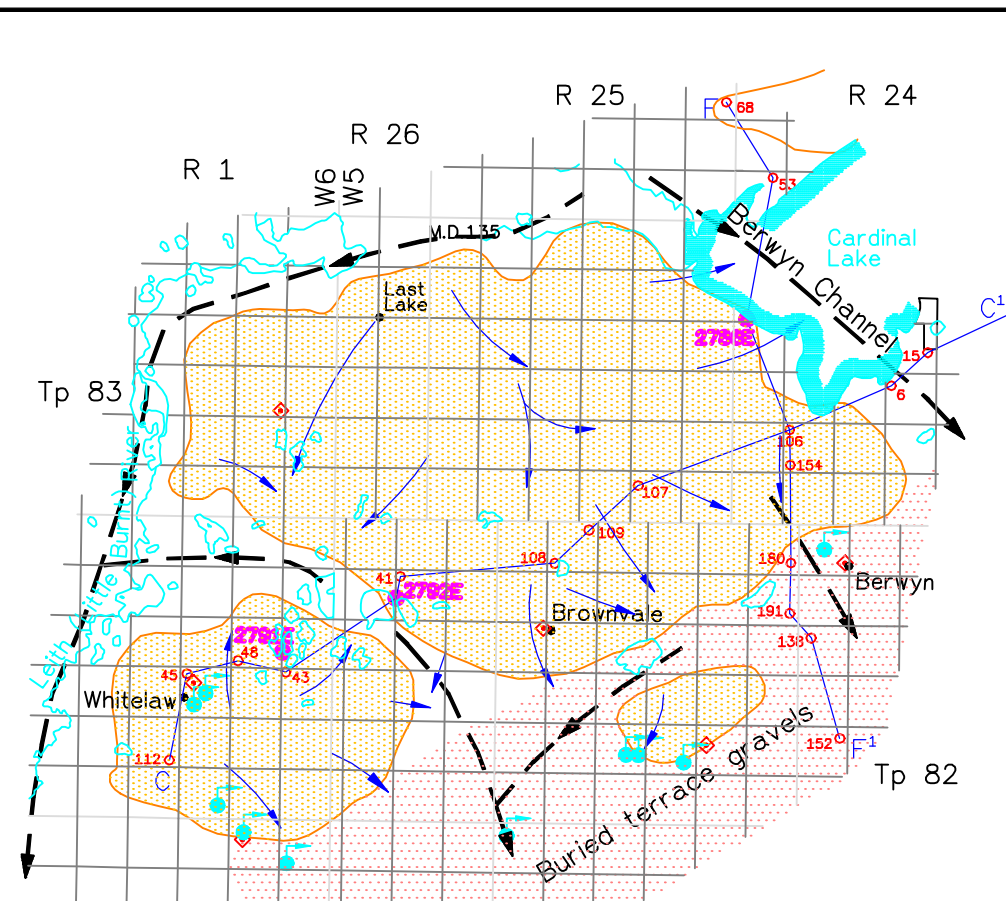
INTERPRETED GROUNDWATER FLOW DIRECTION
