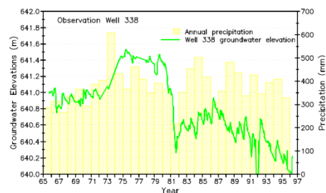
Figure 5b: Water Level and Precipitation Data
